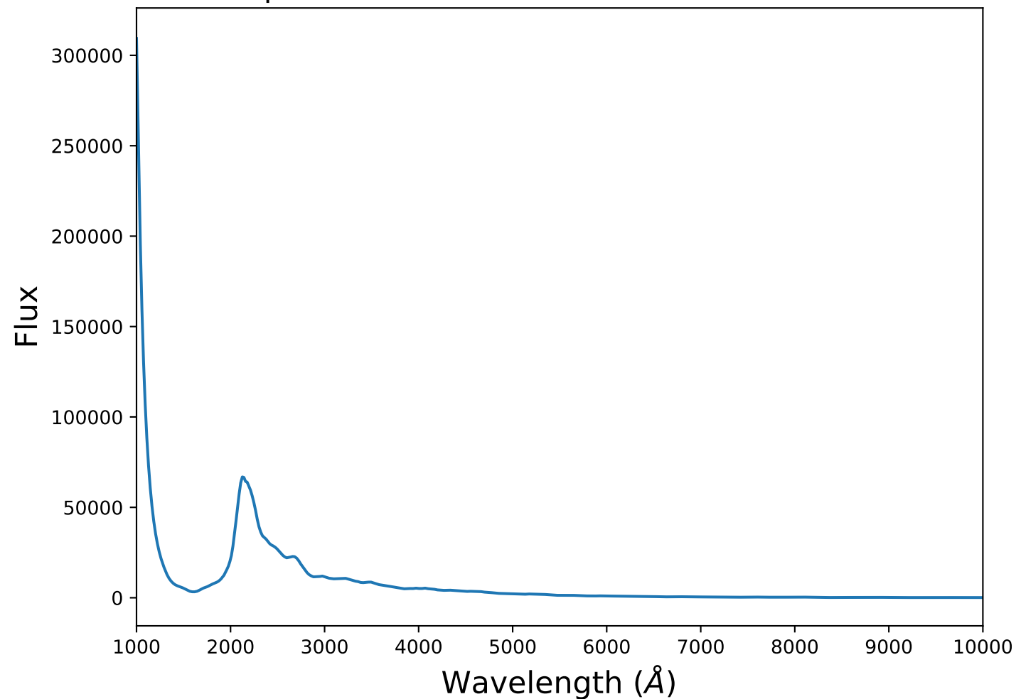
Spectrum 10 for transient SNIa at z=0.47
